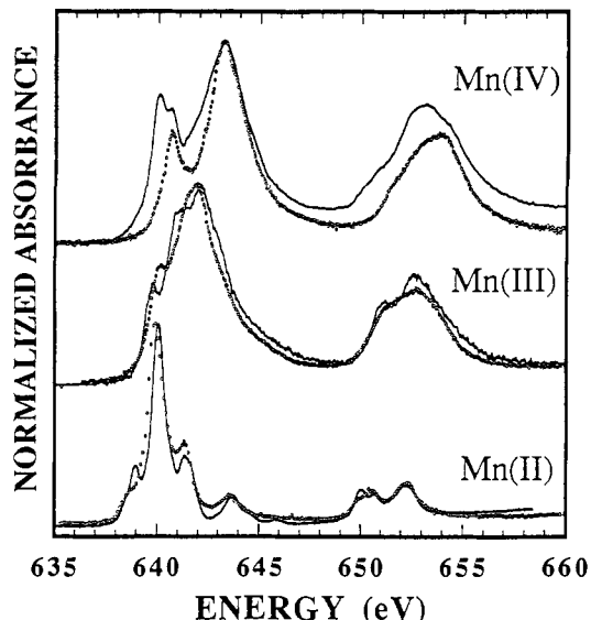
Figure 4. Oxidation data dependence of L-edge position and shape. Top to bottom: (HB(3,5-Me_2pz)_3)_2Mn^{IV}(ClO_4)_2 (—) and Mn^{IV}_2O_2(pic)_4 (···), where pic = picolinate anion; piemontite- Ca_2(Mn^{III},Fe^{III},Al)_2AlO-OH[Si_2O_7][SiO_4] (—) and Mn^{III}(acen)(NO_2) (···), where acen = N,N' -ethylenebis(acetylacetonate imine); Mn^{II}Fe_2 (—) and [Mn^{II}_2(HL)(Cl)_2](ClO_4)_2 \cdot 2dmf \cdot H_2O (···), where H_2L = 1,7,14,20 -tetramethyl-2,6,15,19-tetraaza[7,7](2,6)-pyridinophane-4,17-diol. The spectrum of the first Mn(IV) complex appears to be contaminated by a small amount of its Mn(II) precursor complex. Energy calibration arbitrarily used MnF_2 maximum as 640 eV.
