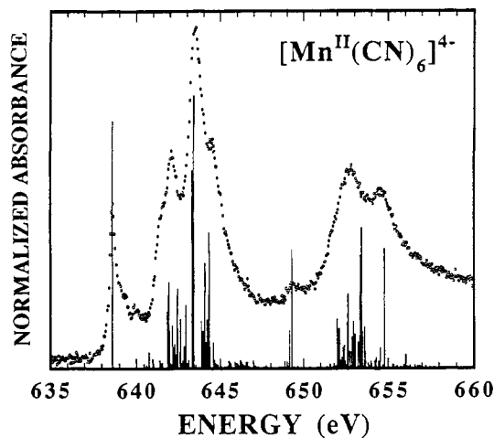
Figure 3. Experimental (OOO) L_{2,3} -edge spectrum for K_4Mn(CN)_6 , compared with the stick diagram showing relative oscillator strengths of individual transitions before instrumental and line width broadening, calculated with 10Dq = 3.9 eV.
